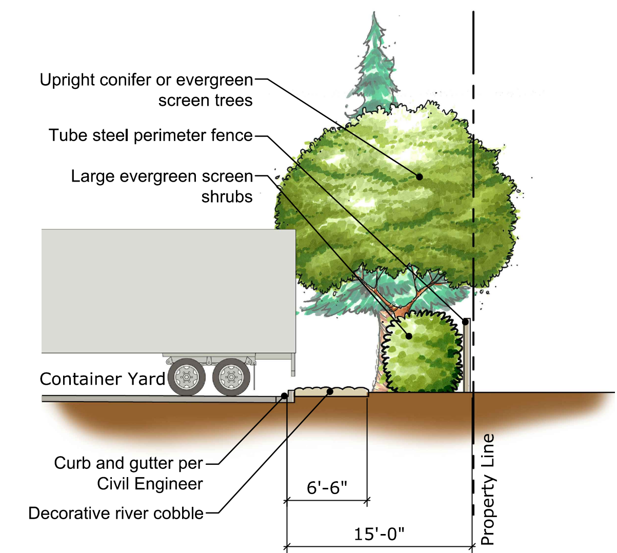
Section 'C'
