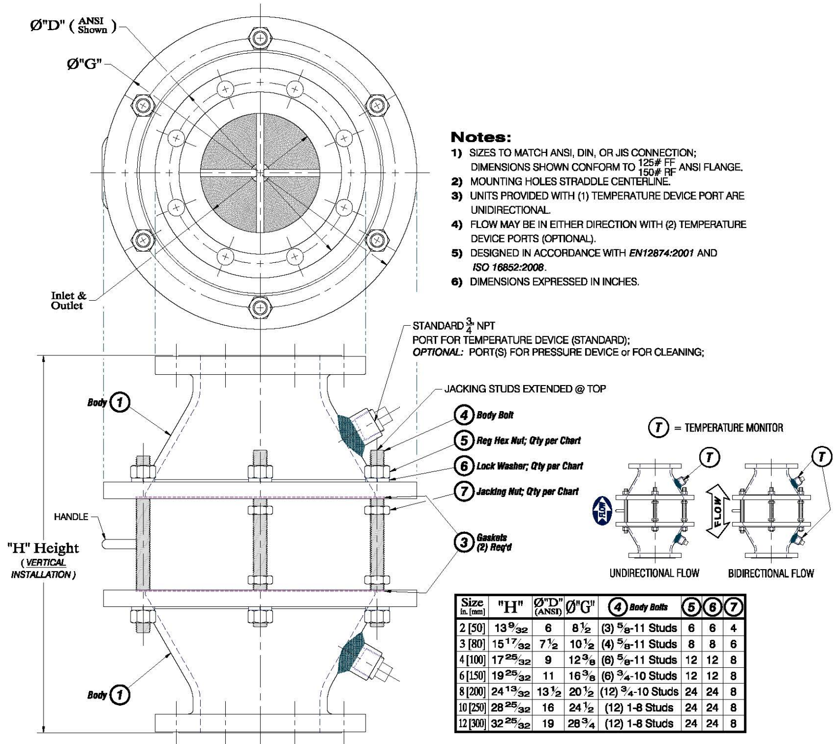
Figure 3. Model 94406 Assembly
