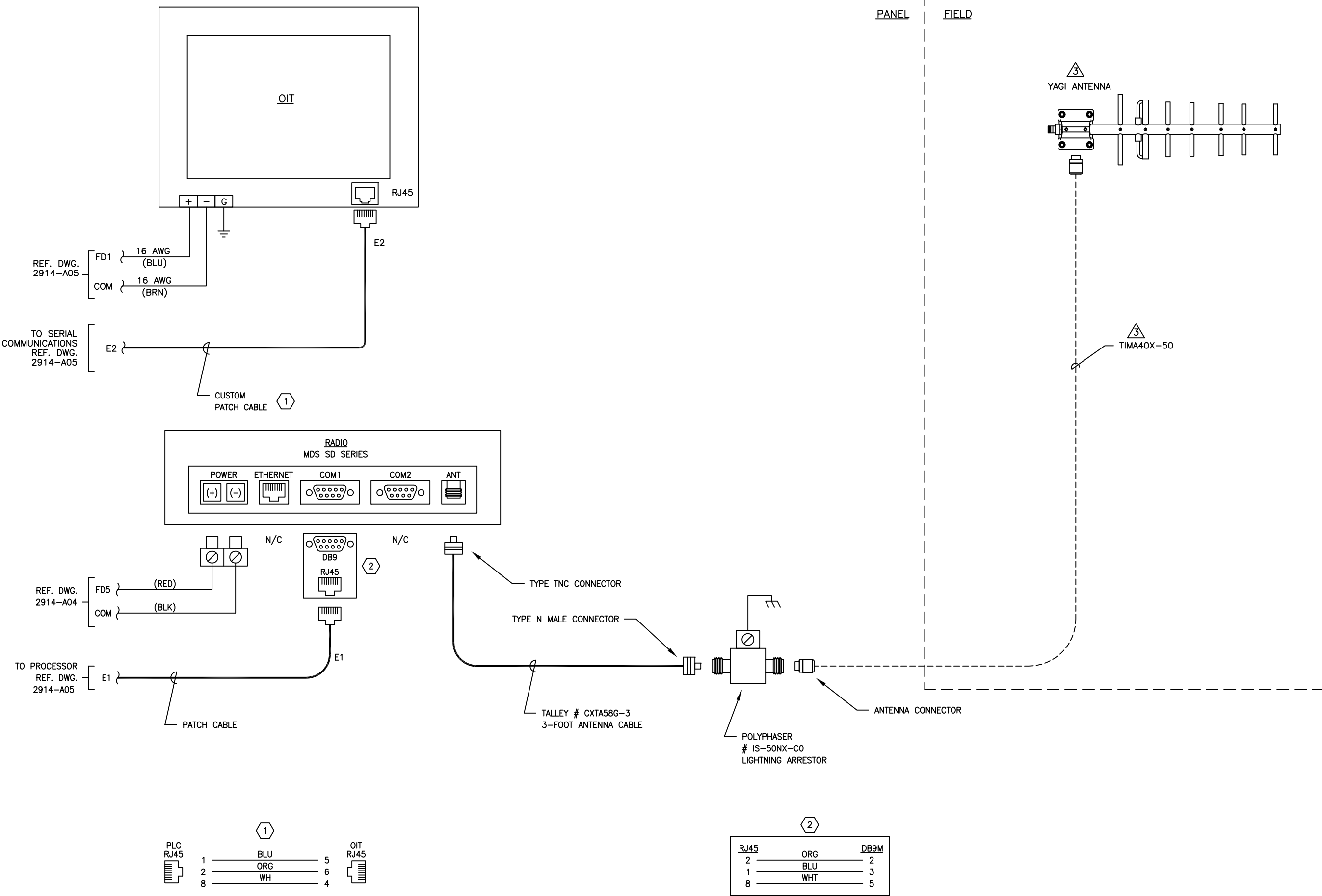
OIT TO PLC CONNECTION DIAGRAM
