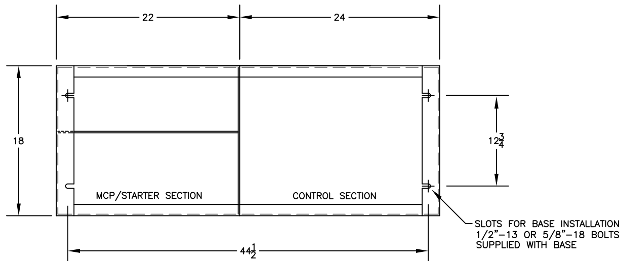
BOTTOM VIEW MOUNTING SLOT DETAIL
