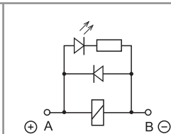
C: Option 6, 7, 74 LED + diode (DC, polarity positive to pin A/A1)
