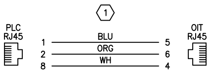
OIT TO PLC CONNECTION DIAGRAM
