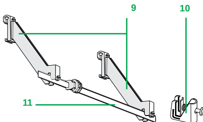
Shielding connection kits
