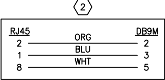
PLC TO RADIO CONNECTION DIAGRAM
