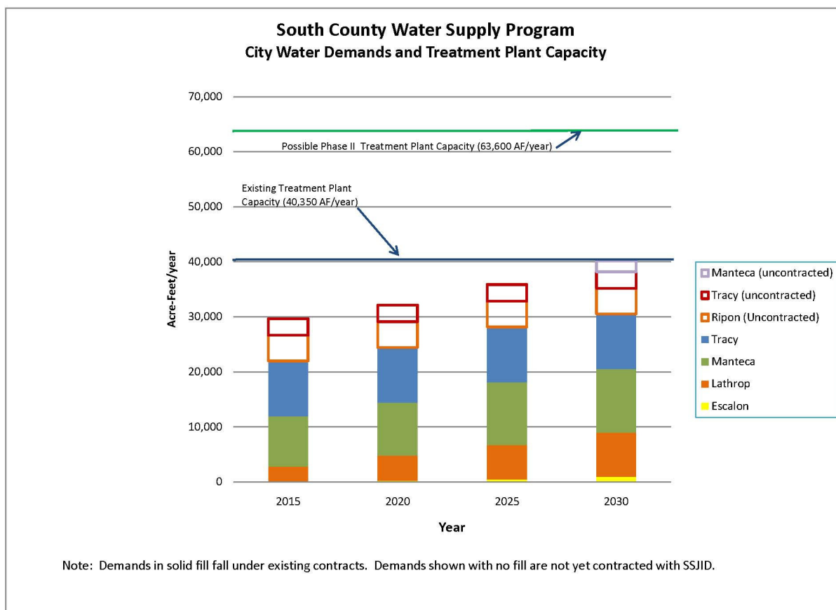
Figure 2 – Future Water Demands and Treatment Plant Capacity
