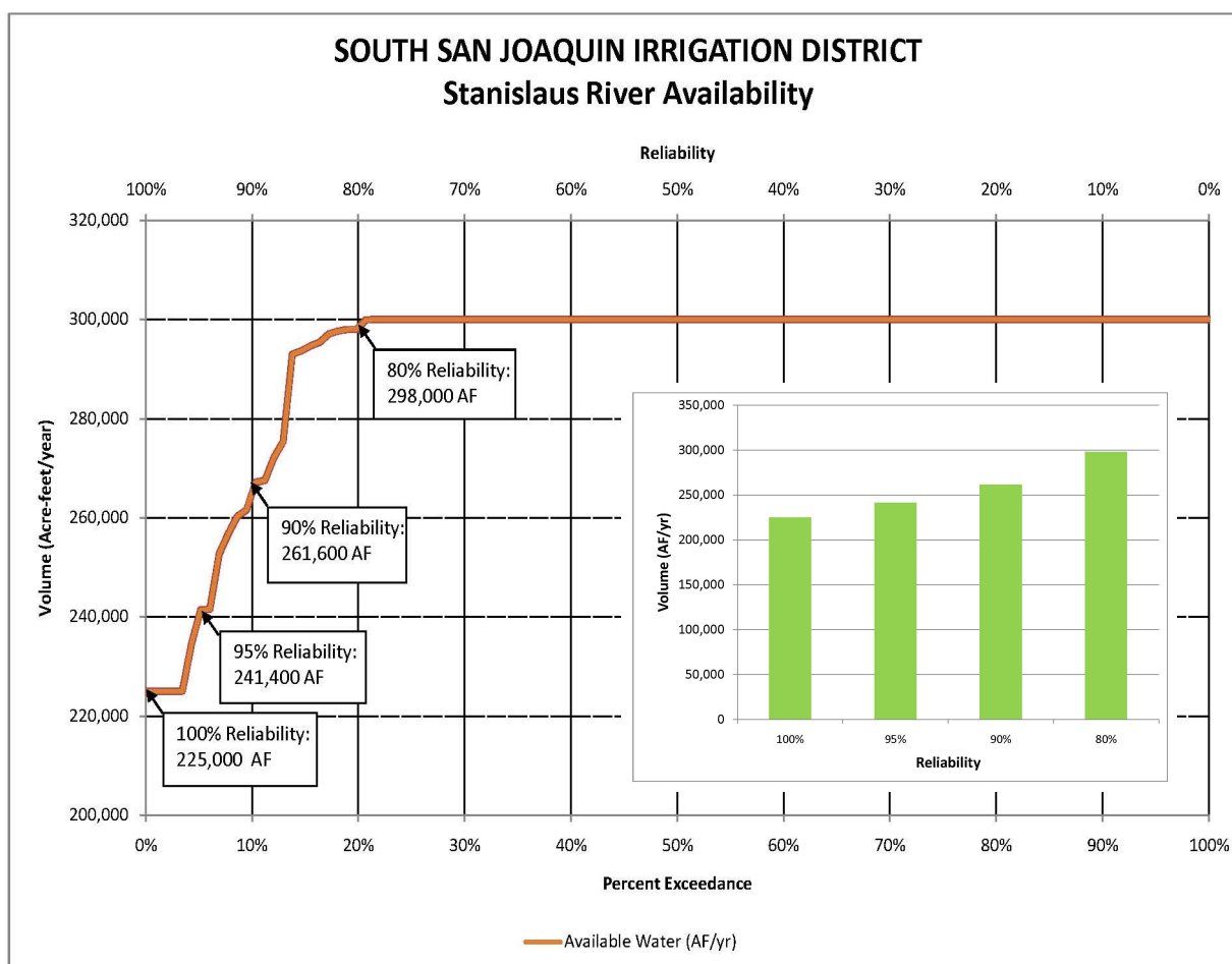
Figure 3 – Water Supply Reliability
